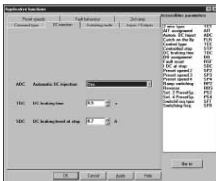
Adjustment of the "d.c. injection" function using the PowerSuite software workshop for PC
